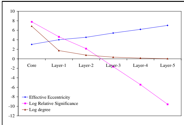
Figure 7: The average importance of each layer: log of the average degree, average effective eccentricity and log of the average relative significance (Int-07-2003 instance)
