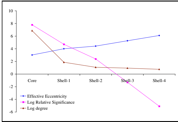
Figure 8: The average importance of each shell: log of the average degree, average effective eccentricity and log of the relative significance (Int-07-2003).
