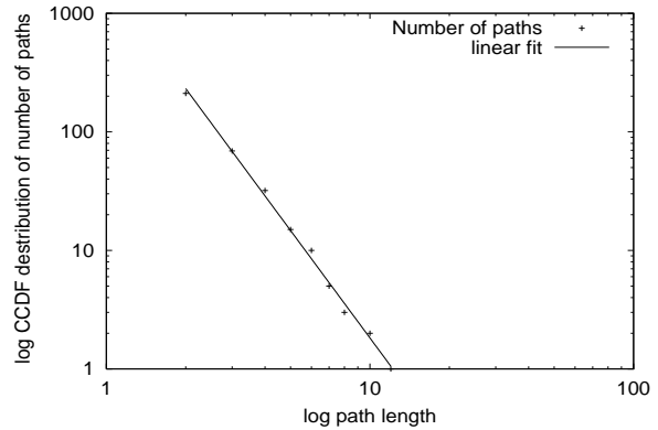
Figure 6: The CCDF distribution of the paths versus the path length between the nodes with degree 590 and 524 in log-log scale (Int-11-97). Correlation coefficient 99.8%.
