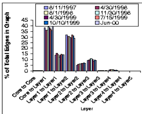
Figure 12: The distribution of edges over time grouped by type.
