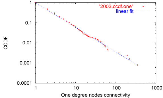
Figure 4: The CCDF of the one-degree neighbors of a node in log-log scale.
