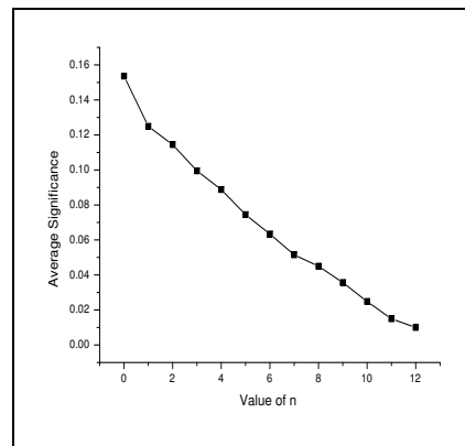
Figure 13: Significance of the core versus relaxing the clique constraint by n edges.
