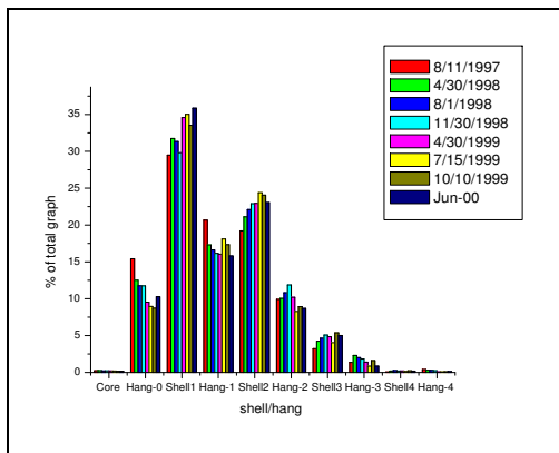
Figure 11: The distribution of nodes over time grouped by class.
