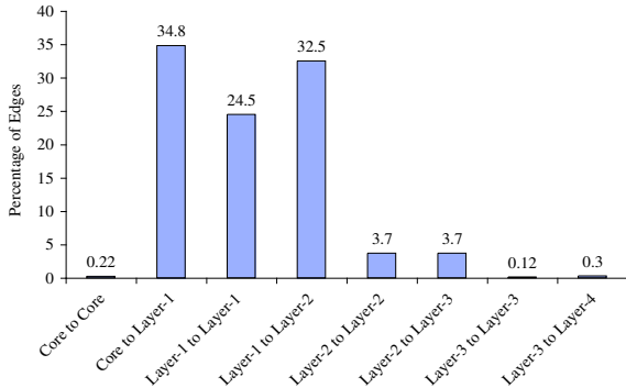
Figure 10: The percentage of the different types of edges classified according to their adjacent nodes (Int-07-2003).
