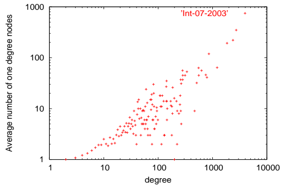
Figure 3: The average number of one-degree neighbors versus the degree of such node.
