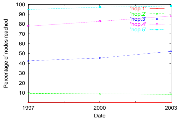
Figure 5: Percentage of nodes reached versus date for the topological paths. Each line represents the percentage for different number of hops.
