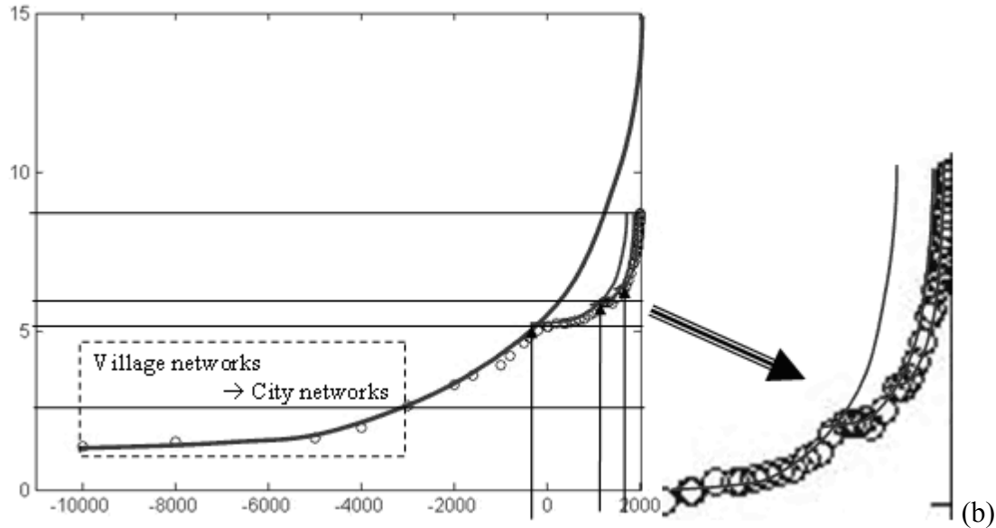
Figure 3: World Population Power-Law Growth Spurts and Flattening as shown in: (a) von Foerster et al.'s (1960, redrawn) log-log plot with updated population estimates back to 1 million years BCE, with downward arrows marking the start of reduced growth rates, and (b) a semilog plot of the same data with successive power-law fits
