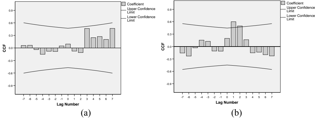
Figure 8: Time-lagged cross-correlation effect (a) of Mid-Asia q on Europe and (b) of the silk road trade on European \beta (ten top cities)
